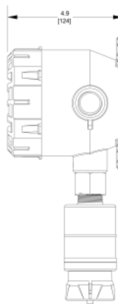
Figure 52 Deep Lid Depth with M25 Adapter
