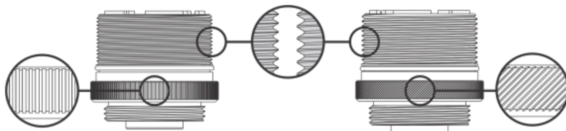
Figure 45 Digital Sensor for Div 1 & 2, Zone 1 & 2 (Left) vs Digital Sensor for Div 2, Zone 2 only (right)
