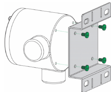
Figure 16 JB5000 Bracket Attachment
