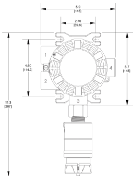
Figure 50 ULTIMA X5000 Height & Width with M25 Adapter
