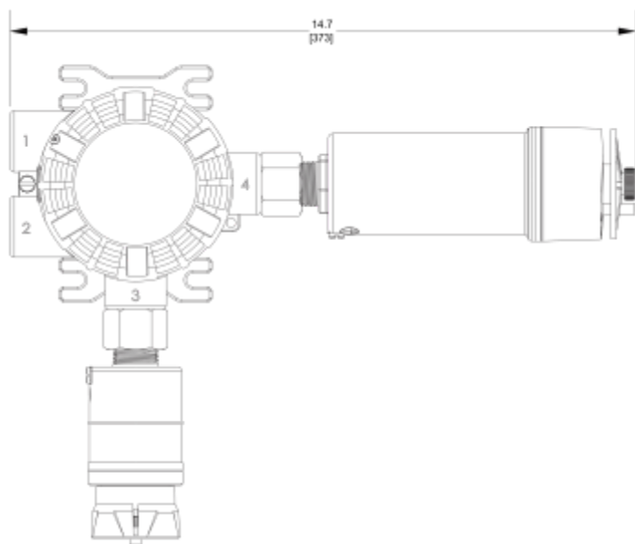
Figure 53 ULTIMA X5000 Width with XIR PLUS Sensor with M25 Adapter
