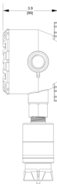
Figure 51 Short Lid Depth with M25 Adapter
