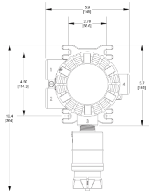
Figure 46 ULTIMA X5000 Height & Width
