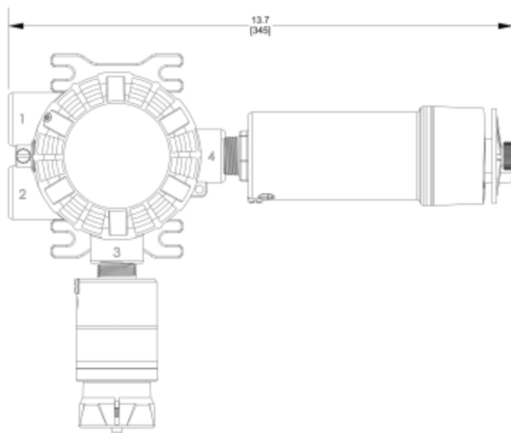
Figure 49 ULTIMA X5000 Width with XIR PLUS Sensor
