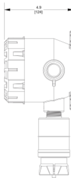
Figure 48 Deep Lid Depth
