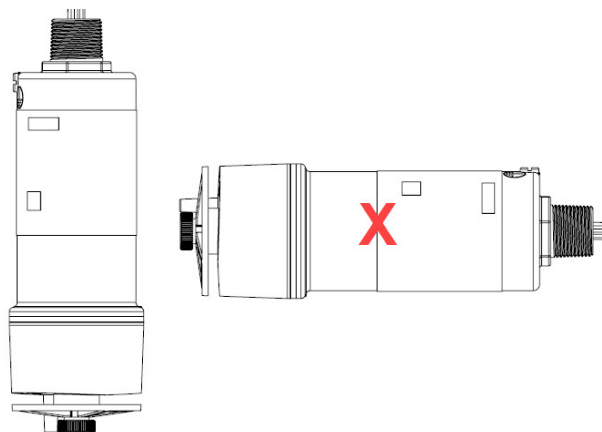
Figure 10 Correct and Incorrect Mounting Orientations for IR Sensor
