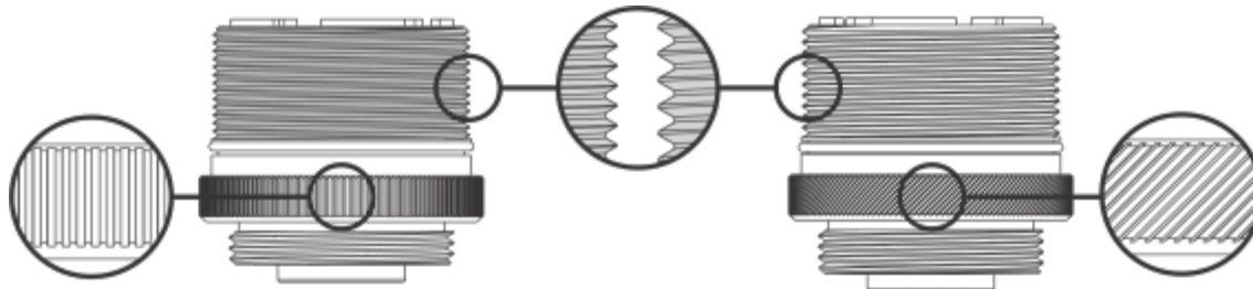
Figure 37 Digital Sensor for Div 1 & 2, Zone 1 & 2 (Left) vs Digital Sensor for Div 2, Zone 2 only (right)
