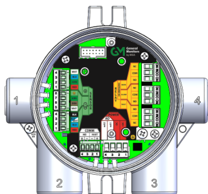
Figure 28 PC Board with Relays
