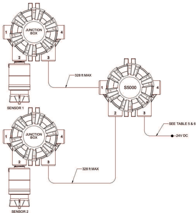
Figure 26 Remote Sensors
