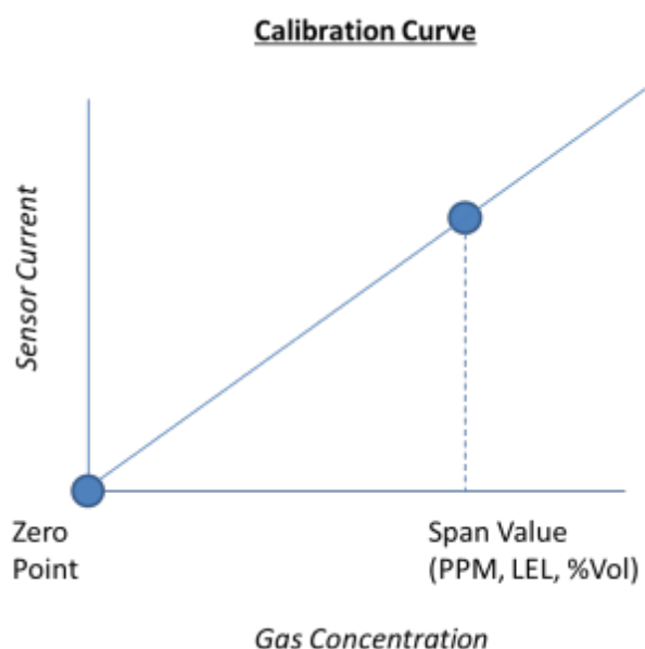
Figure 32 Calibration Curve
