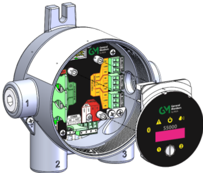
Figure 12 Terminal Connections
