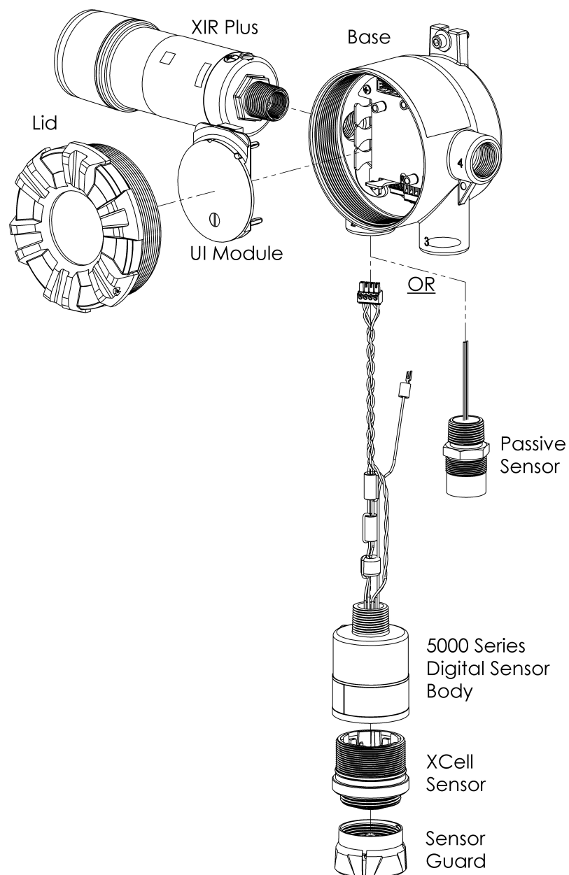
Figure 3 Exploded View
